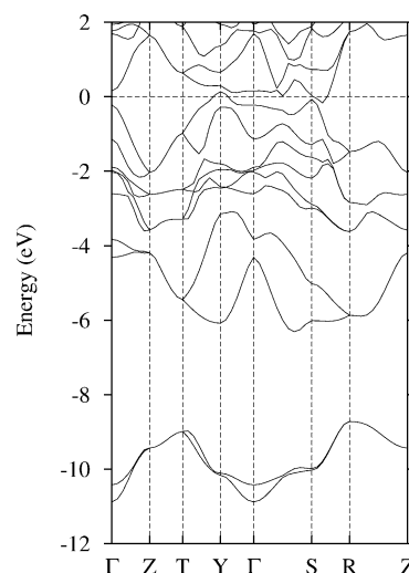
Figure 3. Band structure of YAlC within density functional theory.
