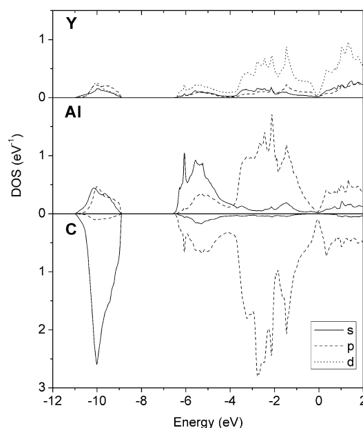
Figure 2. Partial density of states of YAlC.
